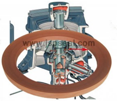
Cone Crusher Dust Ring
